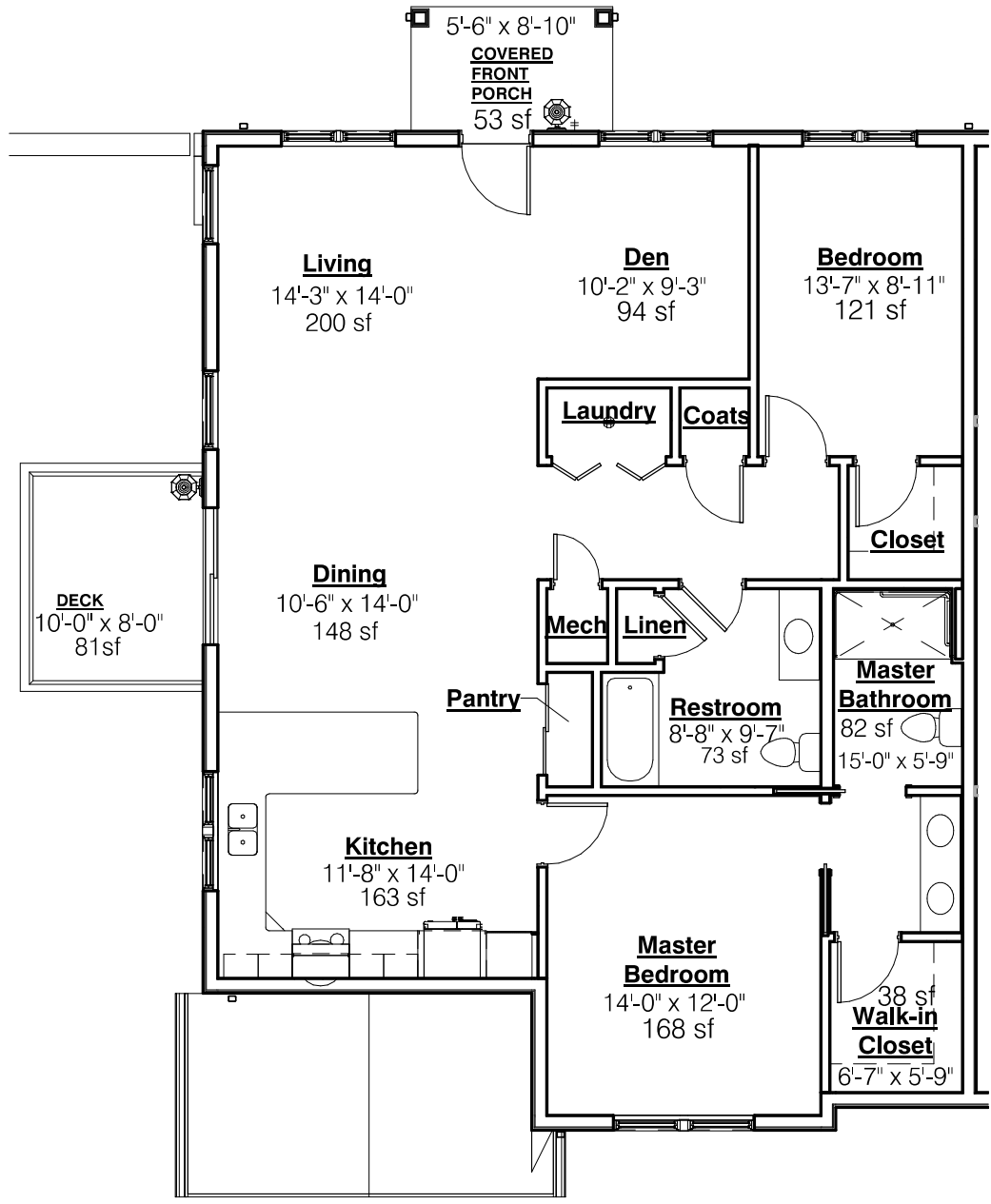
1 | 2 Bedroom 2 Bath with Den - 1,291 SF
